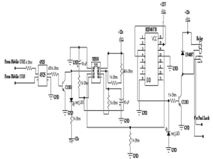
Figure9:3 rd stage of the circuit
