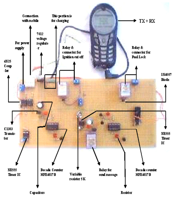
Figure .5: Labeled diagram of Security module
