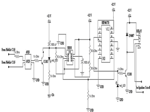
Figure.8:2 nd stage of the circuit
